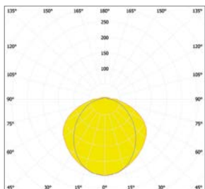
POLAIR DIAGRAM TPN | FROSTED
